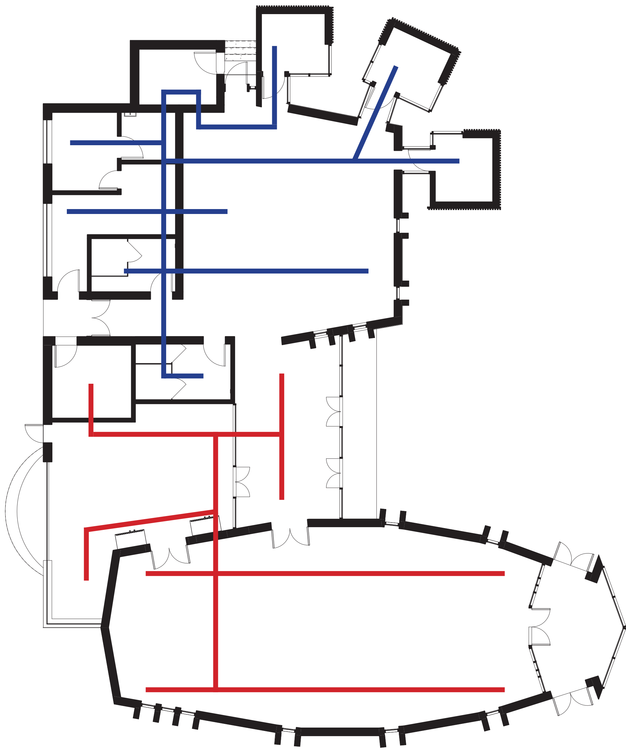
HVAC System Diagram
