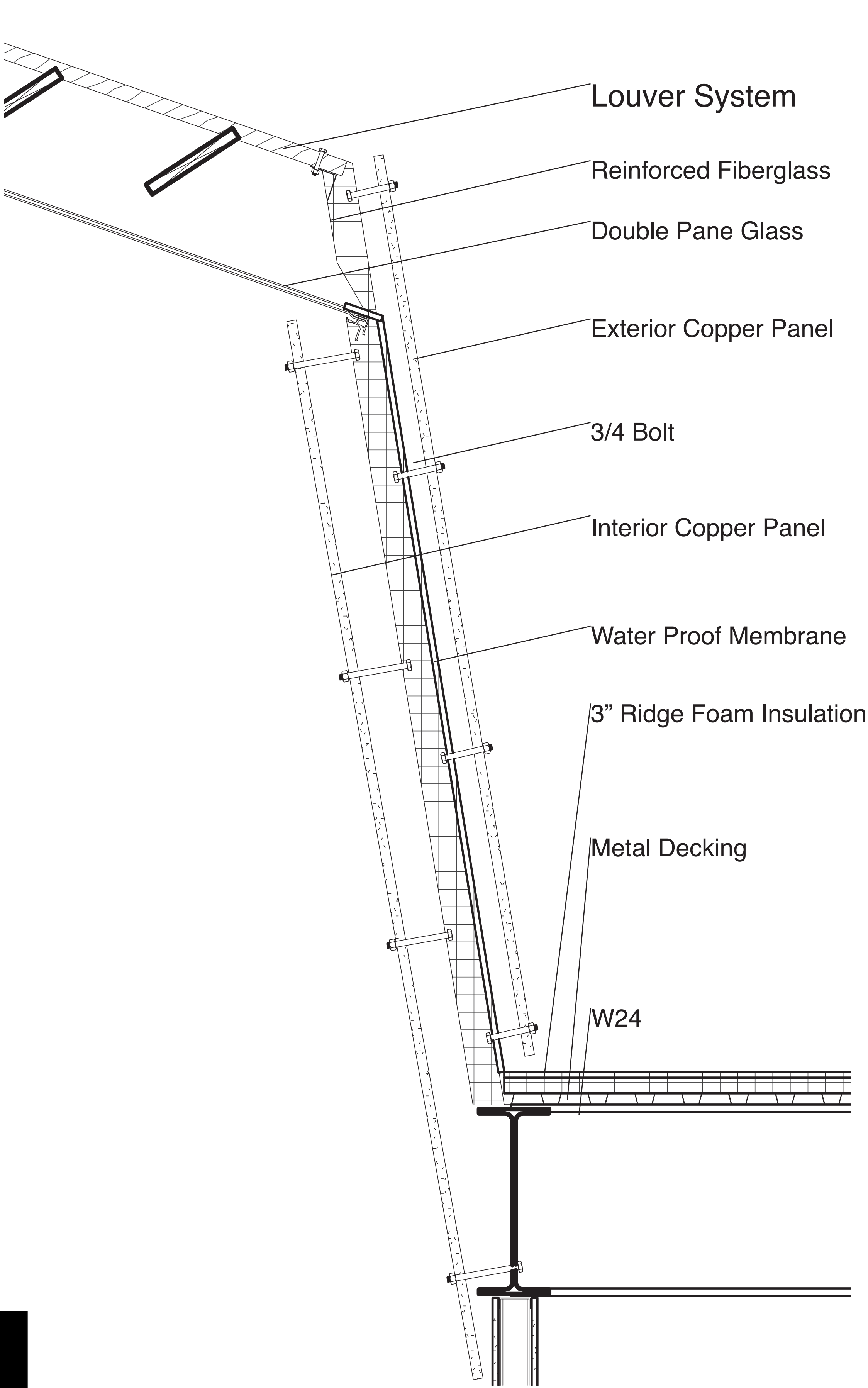
Wall Detail
