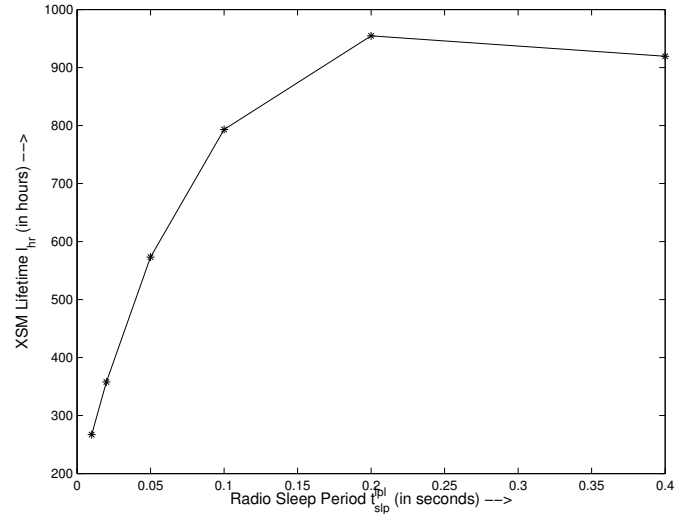
Fig. 4. ExScal network lifetime in the low power listening mode with PIR as the wakeup sensor and in-network data aggregation, as a function of radio sleep period, t_{slp}^{lpl} .
