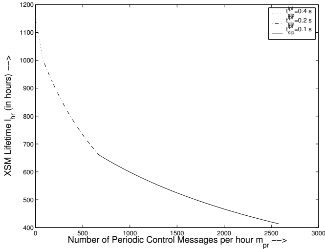
Fig. 3. Optimal ExScal network lifetime in the low power listening mode and hierarchical sensing when the number of periodic control messages ( m_{ppr} ) is varied from 0 to 2580 messages per hour.
