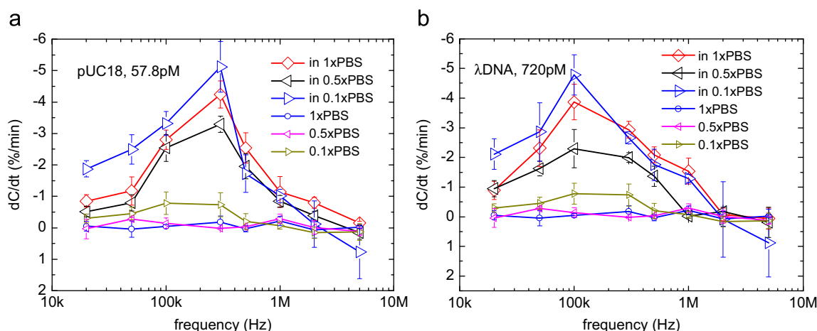
Fig. 6. Capacitance change rate of unlabeled DNA in diluted PBS. (a) Capacitance change of pUC18 in diluted PBS (b) capacitance change of \lambda DNA in diluted PBS.
