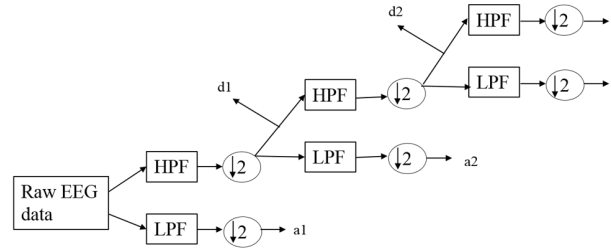
FIGURE 1. Graphical representation of DWT decomposition. (HPF: High pass filter, LPF: Low pass filter.)
