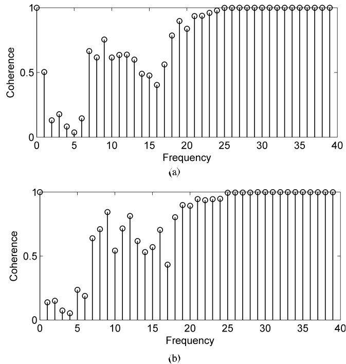
FIGURE 8. Magnitude squared coherence measure plot for one subject from AF3 location after denoising with (a) DWT+ST+coif3 (b) DWT+ST+bior4.4 combination.
