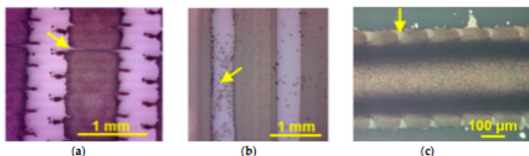
Figure 11. IJP Ag trace printing issues: (a) Micro-gap on traces resulting discontinuity; (b) misfired droplets due to partially blocked nozzles; and (c) rugged edges of a printed traces.
