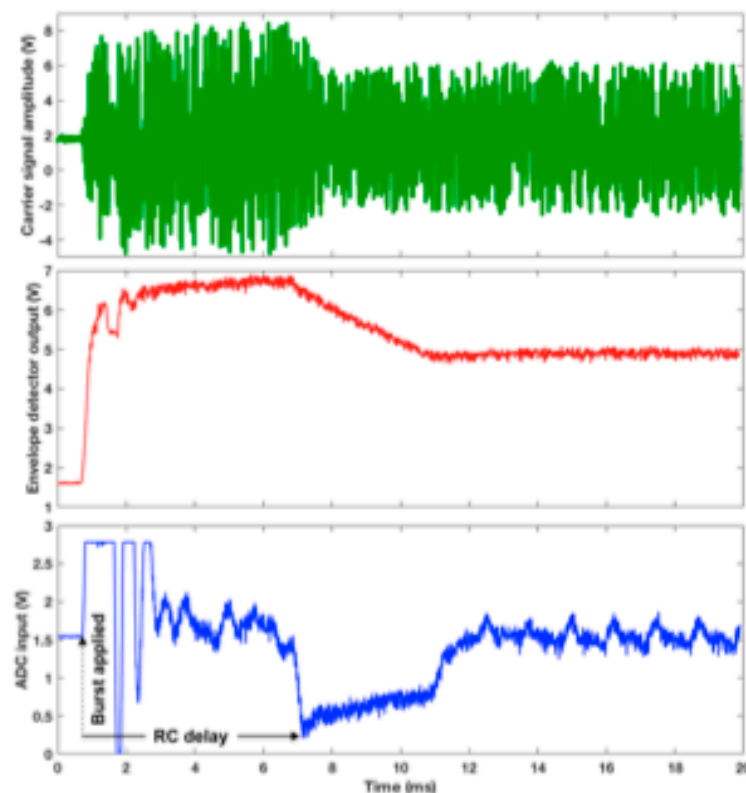
Figure 13. WRAP temperature sensor response captured by an oscilloscope for various stages of the signal during a burst applied to capture data from the sensor: (top) Carrier signal at the scanner coil, (middle) signal at the envelope detector, and (bottom) signal at the input of the ADC.
