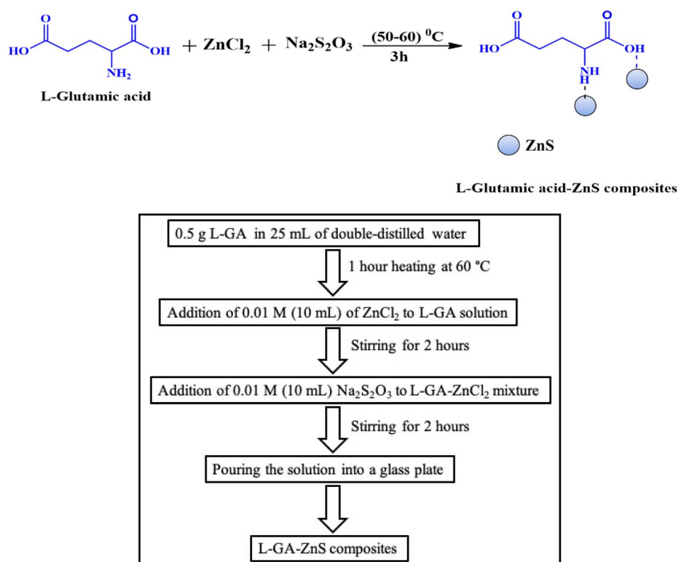
Fig. 1 Schematic illustration and reaction scheme for the synthesis of L-GA/ZnS composites.
