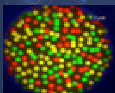
Quantum Dots
