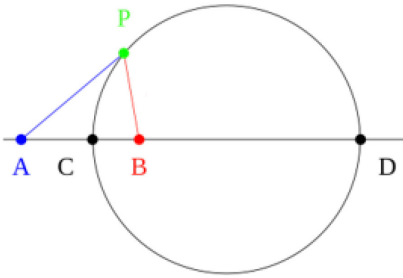
(A) Apollonian circle definition for the L^2 metric in which P represents the point that has a ratio constant for c = \frac{d_2(P,A)}{d_2(P,B)} .
