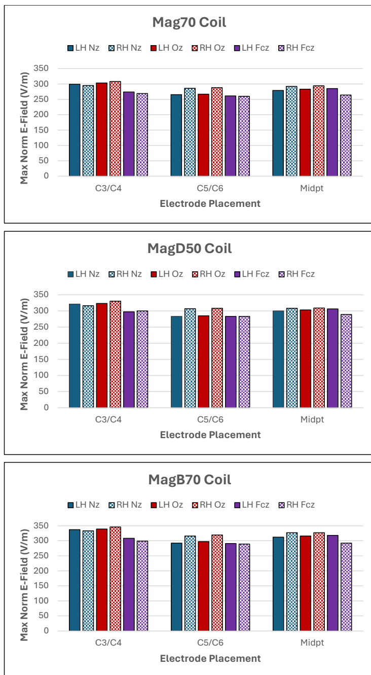
Figure 4. The max norm E-field at the electrode placements and orientation for the three different coils, (A) Mag70, (B) MagD50, (C) MagB70.
