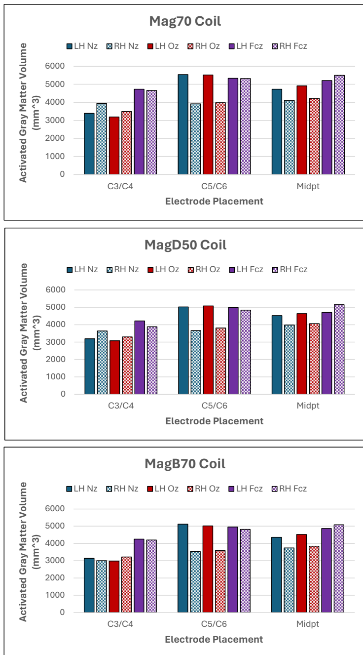
Figure 5. The activated gray matter volume at the electrode placements and orientation regarding coils, (A) Mag70, (B) MagD50, (C) MagB70.
